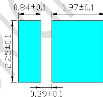
Recommended PCB solder PAD
