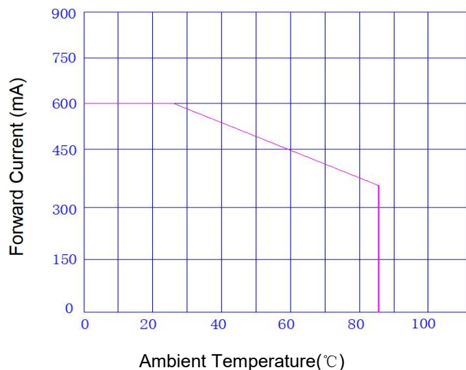
Fig.2- Forward Current vs. Ambient Temp
