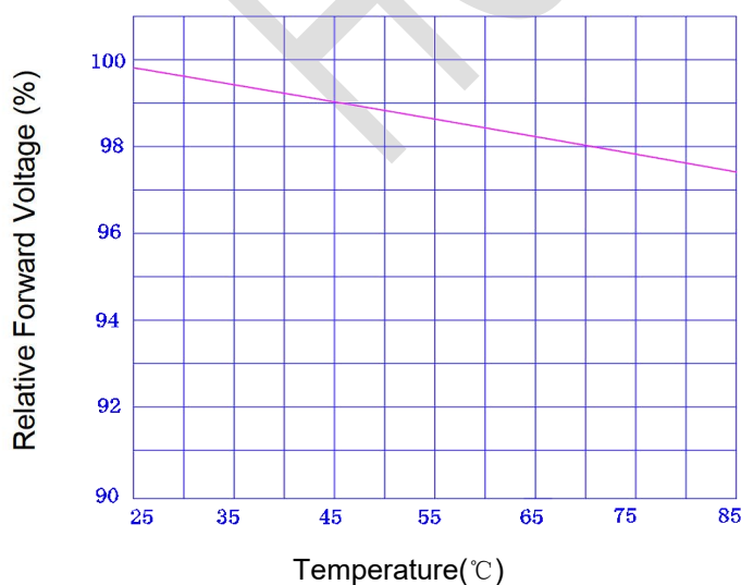
Fig.6- Relative Forward Voltage vs. Temperature
