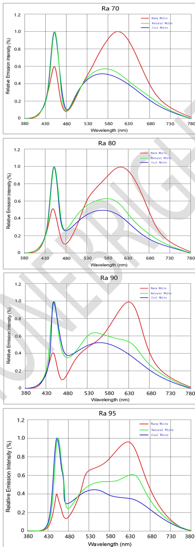
Fig.1-Spectrum Distribution
