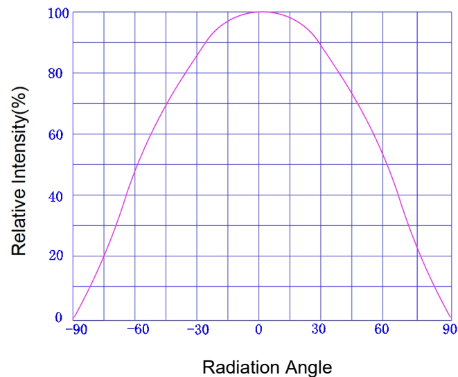
Fig.7- Directivity
