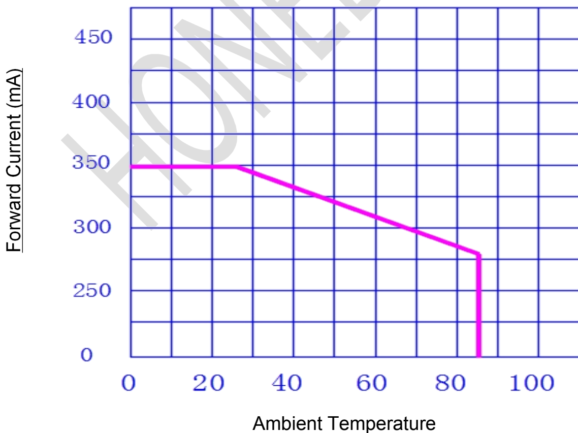
Fig.2- Forward Current vs. Ambient Temp.
