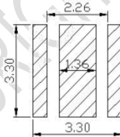
Recommended PCB solder PAD
