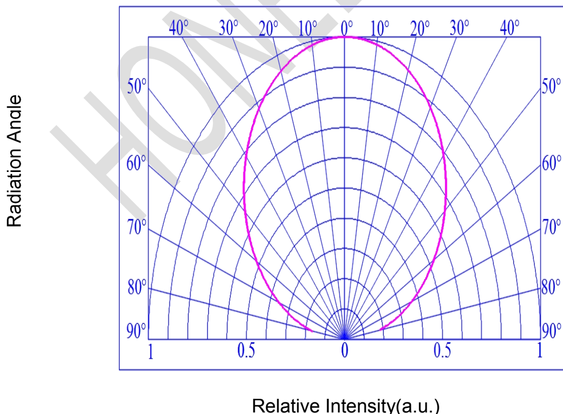
Fig.6- Directivity
