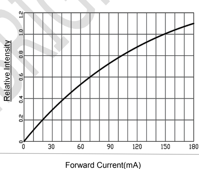
Fig.4- Relative Intensity vs. Forward Current
