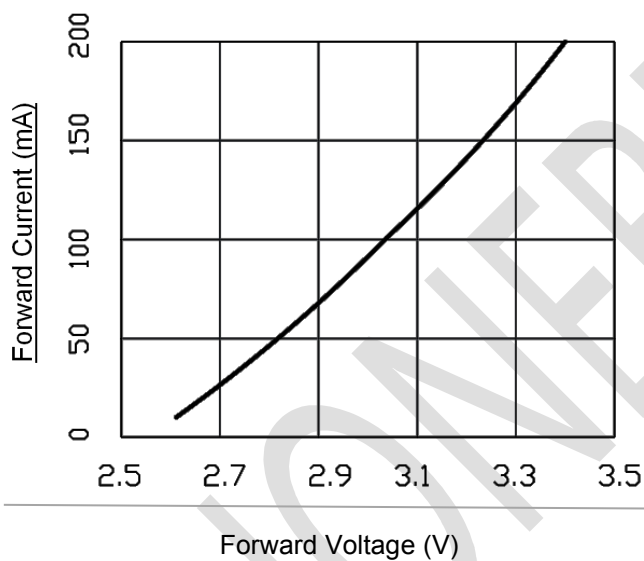
Fig.3-Forward Current vs. Forward Voltage
