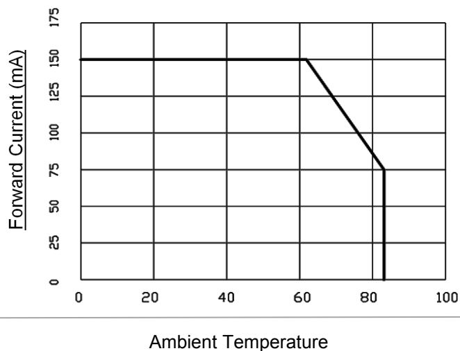
Fig.6- Forward Current vs. Ambient Temp.
